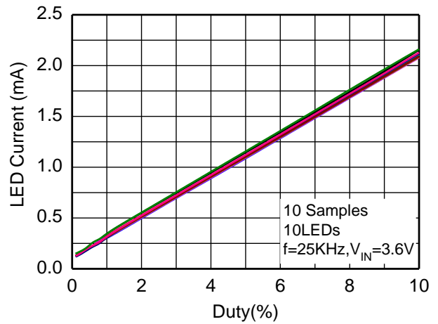
PWM Dimming Distribution
