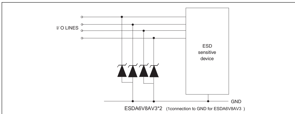
Figure4: ESDA6V8AV3 protection against ESD
